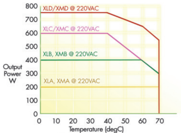
XLA/XLB/XLC/XLD and XMA/XMB/XMC/XMD @ 220VAC Derating
