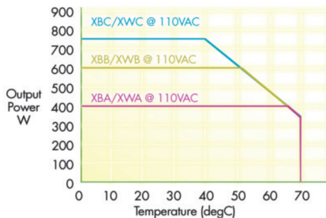
XBA/XBB/XBC and XWA/XWB/XWC @ 110VAC Derating
