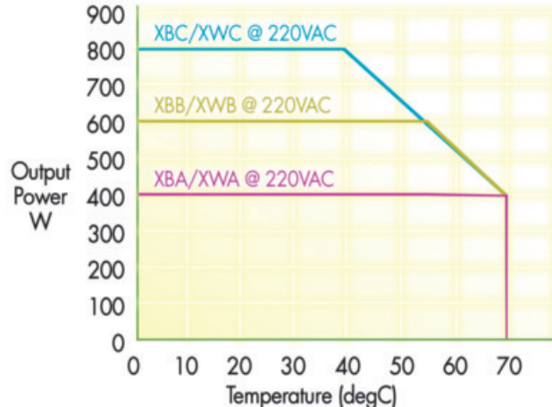
XBA/XBB/XBC and XWA/XWB/XWC @ 220VAC Derating
