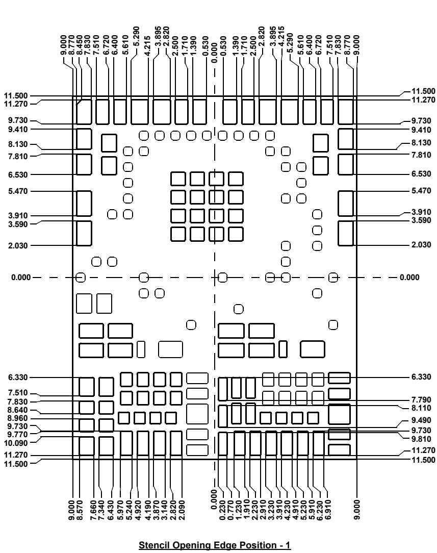
Stencil Opening Edge Position - 1
