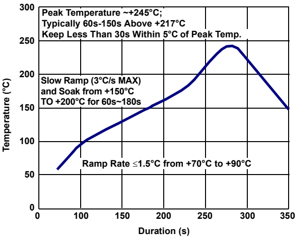
Figure 25. Typical Reflow Profile
