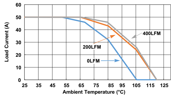
Figure 26. 12V IN to 5V OUT , f SW = 571kHz
