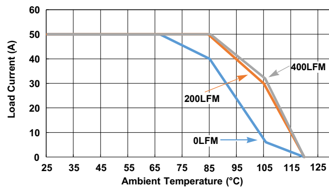
Figure 25. 12V IN to 3.3V OUT , f SW = 533kHz
