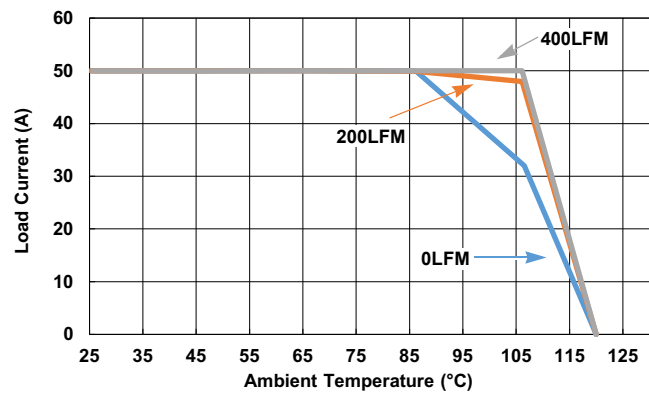
Figure 20. 5V IN to 1.5V OUT , f_{\text{SW}} = 471\text{kHz}
