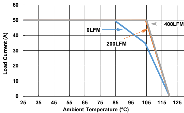
Figure 17. 12V IN to 1V OUT , f_{\text{SW}} = 364\text{kHz}
