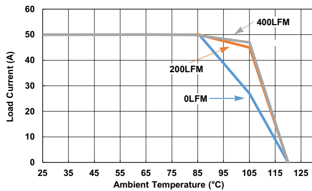
Figure 19. 12V IN to 1.5V OUT , f_{\text{SW}} = 471\text{kHz}
