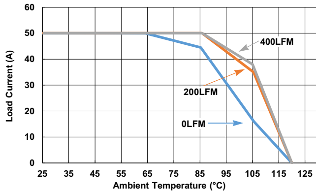
Figure 23. 12V IN to 2.5V OUT , f SW = 533kHz
