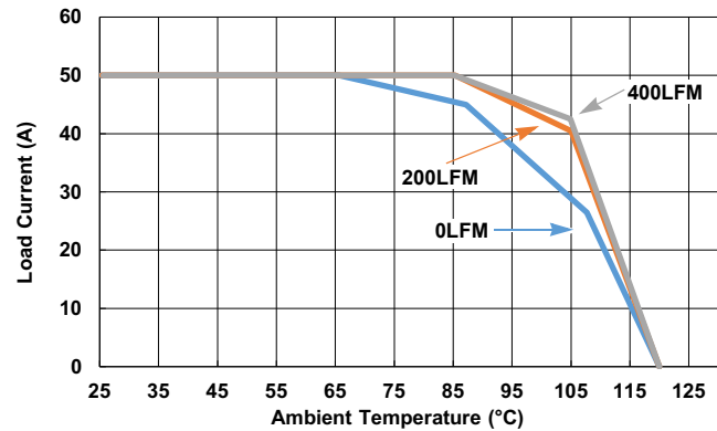
Figure 24. 5V IN to 2.5V OUT , f SW = 533kHz
