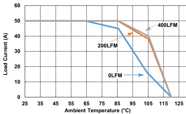
Figure 21. 12V IN to 1.8V OUT , f_{\text{SW}} = 727\text{kHz}
