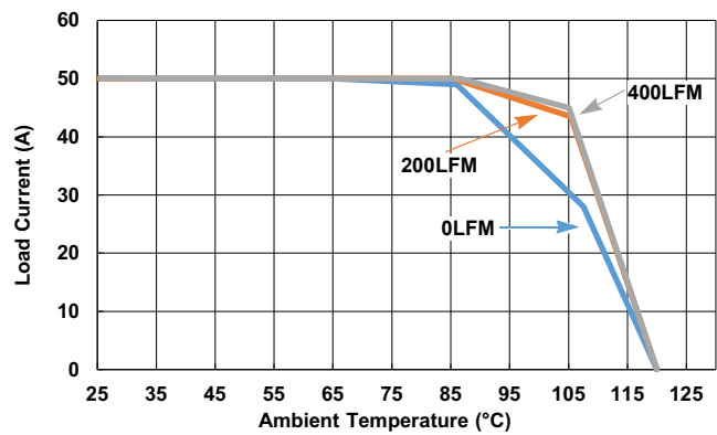
Figure 22. 5V IN to 1.8V OUT , f_{\text{SW}} = 727\text{kHz}
