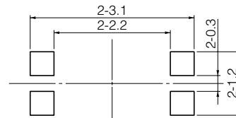
Stencil mask plan
