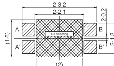
Land pattern plan
